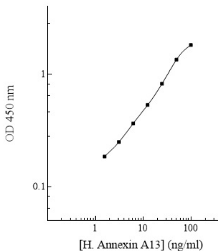
Human Annexin A13 Standard Curve
