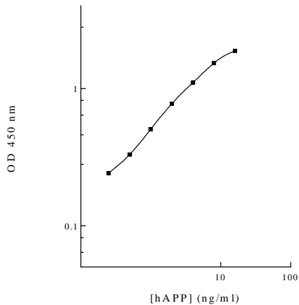
Human APP Standard Curve
