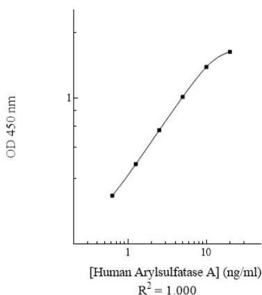
Human Arylsulfatase A Standard Curve
