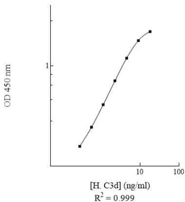
Human Complement C3d Standard Curve
