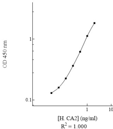
Human CA2 Standard Curve
