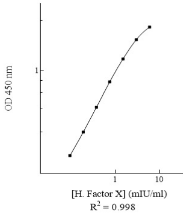
Human Factor X Standard Curve
