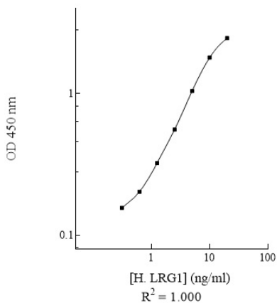
Human LRG1 Standard Curve
