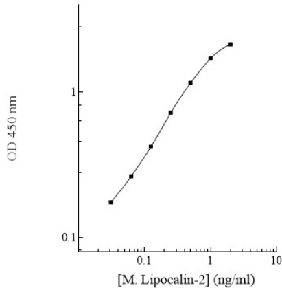
Mouse Lipocalin-2 Standard Curve
