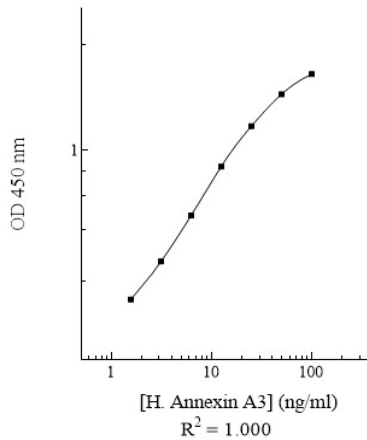
Human Annexin A3 Standard Curve
