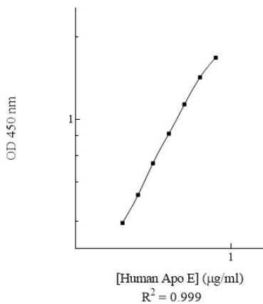
Human Apo E Standard Curve
