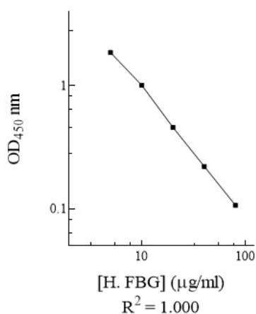
Human FBG Standard Curve
