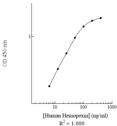
Human Hemopexin Standard Curve
