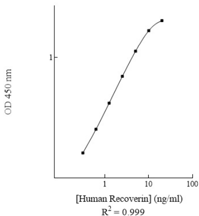
Human Recoverin Standard Curve
