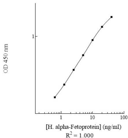
Human alpha-Fetoprotein Standard Curve
