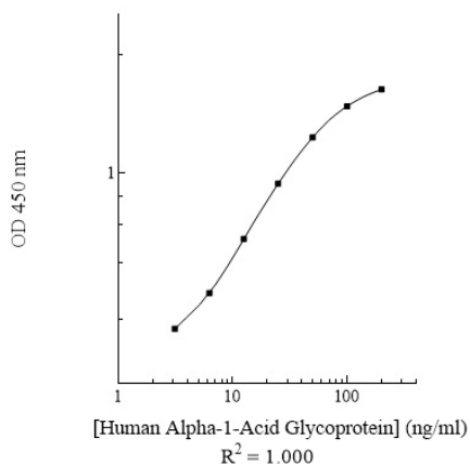
Human Alpha-1-Acid Glycoprotein Standard Curve
