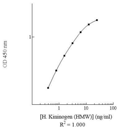
Human Kininogen (HMW) Standard Curve
