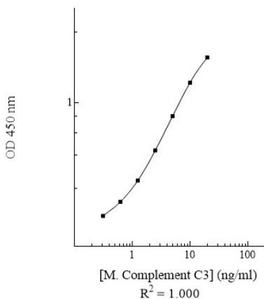
Mouse Complement C3 Standard Curve
