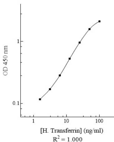
Human Transferrin Standard Curve
